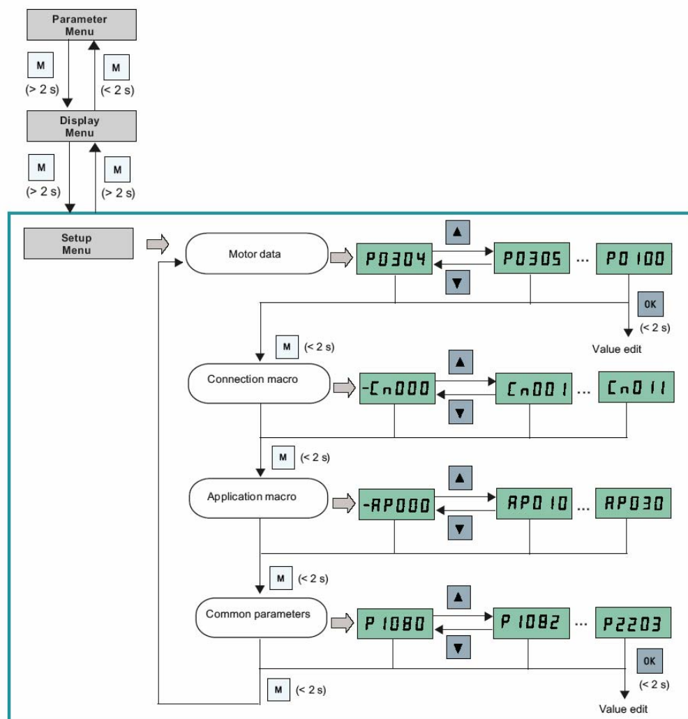
Menu structure
